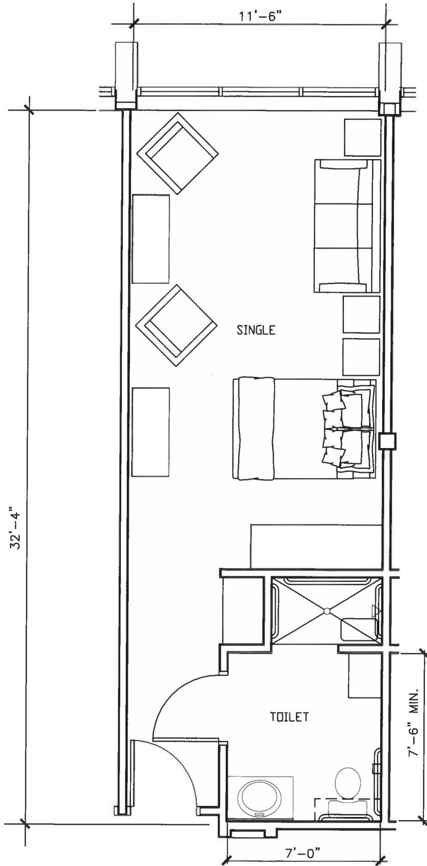
"CONTINENTAL" 372 SQUARE FEET
